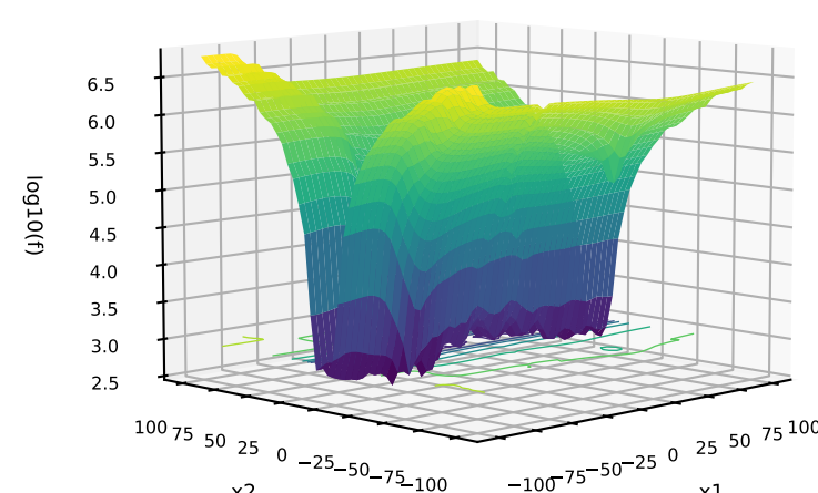
87: C=DPM-BGSOFTMAX; P=MIXED; T=MIXED G=Rosenbrock+StepRastrigin+Griewank BuecheRastrigin+BentCigar+LinearSlope
