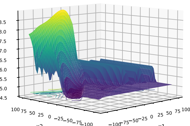
400: C=CPM-PMEAN; P=MIXED; T=ROT G=StyblinskiTang+Katsuura HappyCat+HappyCat
