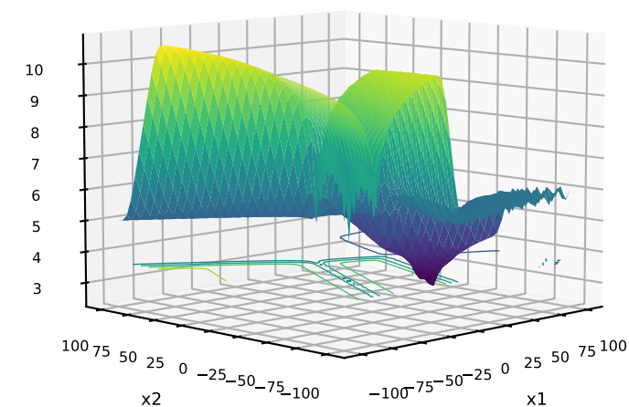
64: C=DPM-SOFTMAX; P=MIXED; T=MIXED G=BentCigar StepRastrigin
