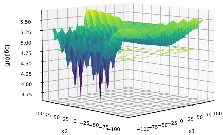
53: C=CPM-PMEAN; P=MIXED; T=MIXED G=GriewankRosenbrock+Gallagher21 Ackley+Katsuura+LinearSlope
