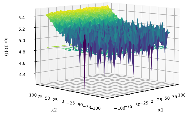
55: C=DPM-BGSOFTMAX; P=MIXED; T=MIXED G=Weierstrass+Exponential+HGBat+BentCigar+Rosenbrock+Ellipsoidal GriewankRosenbrock+BentCigar+StyblinskiTang+SumDifferentPowers
