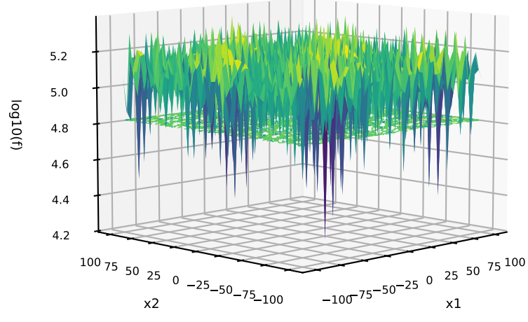
18: C=NONE; P=NONE; T=AFF G=Gallagher21
