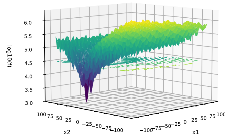
223: C=DPM-SOFTMAX; P=MIXED; T=MIXED G=SchafferF7+BuecheRastrigin HGBat+BentCigar+Gallagher21
