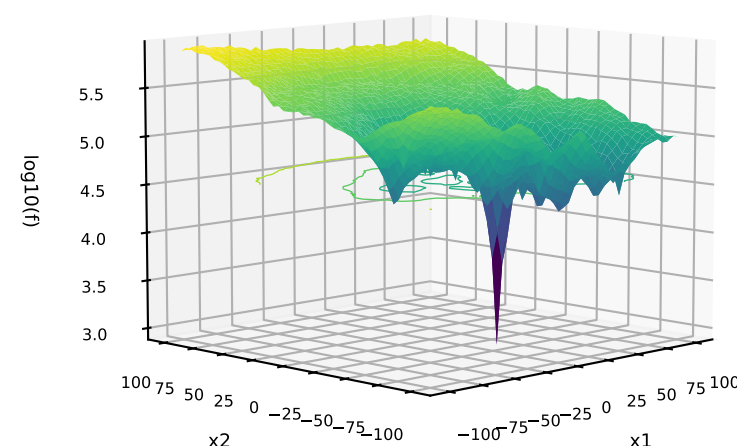
83: C=DPM-BGSOFTMAX; P=MIXED; T=MIXED G=Katsuura+GriewankRosenbrock+SumDifferentPowers+Gallagher21 GriewankRosenbrock+Rosenbrock+Gallagher21+SchafferF7Cond1000
