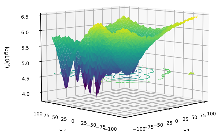
237: C=CPM-LWELL; P=MIXED; T=MIXED G=Levy+HappyCat Weierstrass+Gallagher21
