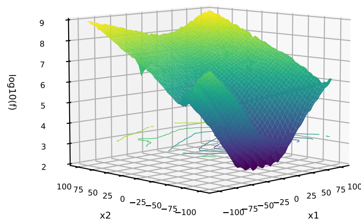
59: C=CPM-SUM; P=MIXED; T=MIXED G=LinearSlope Ellipsoidal+Schwefel
