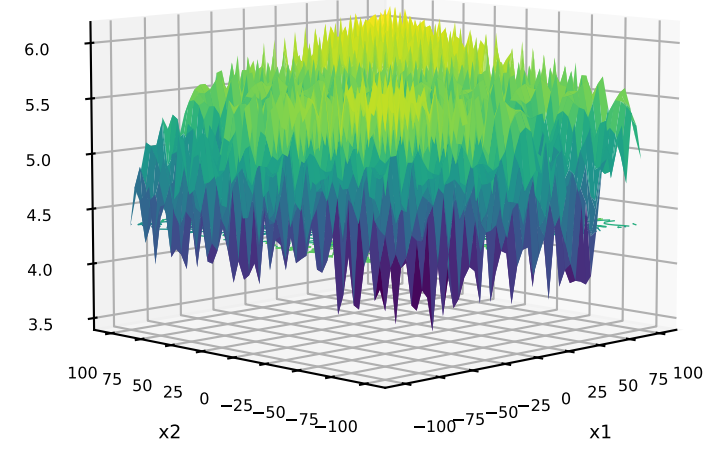
20: C=NONE; P=NONE; T=BROT G=LunacekBiRastrigin
