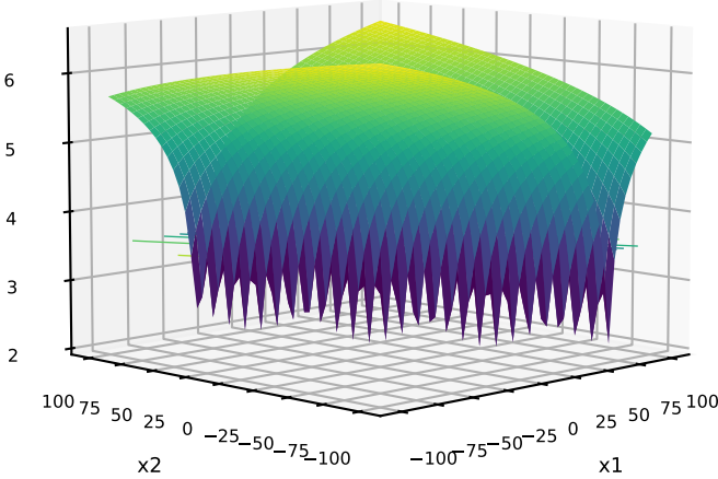
388: C=CPM-PMEAN; P=MIXED; T=MIXED G=BuecheRastrigin+Ellipsoidal+HGBat+Ackley+BentCigar SumDifferentPowers+Weierstrass+BuecheRastrigin+HappyCat+Levy
