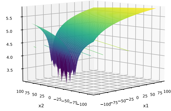
8: C=NONE; P=NONE; T=ROT G=Rosenbrock
