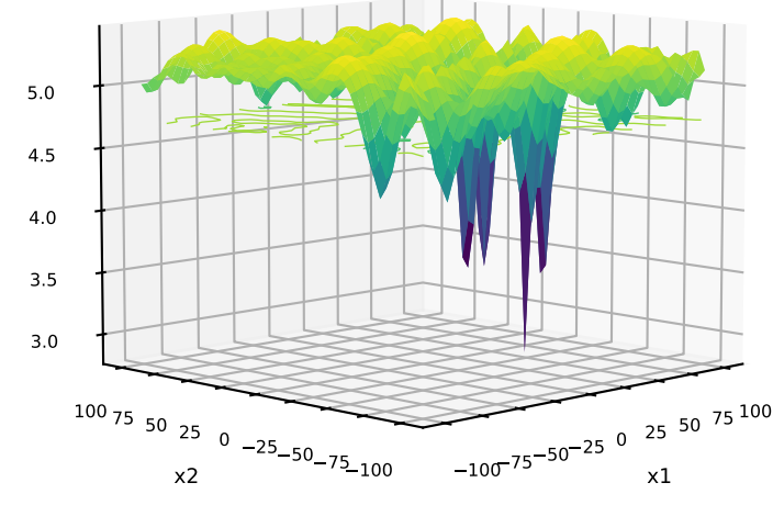
16: C=NONE; P=NONE; T=AFF G=SchafferF7Cond1000
