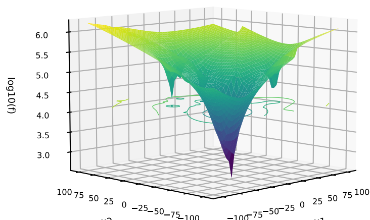
397: C=DPM-SOFTMAX; P=MIXED; T=MIXED G=StepRastrigin+Exponential+BentCigar SumDifferentPowers+BentCigar+BuecheRastrigin
