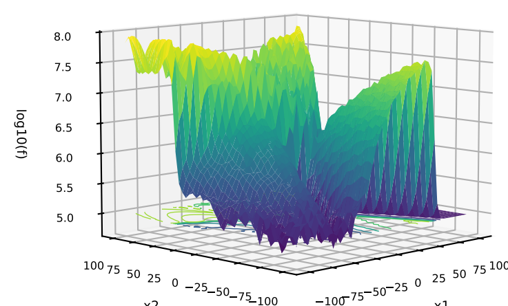
239: C=DPM-SOFTMAX; P=MIXED; T=AFF G=SumDifferentPowers+Schwefel+Griewank StyblinskiTang+Schwefel+Rastrigin
