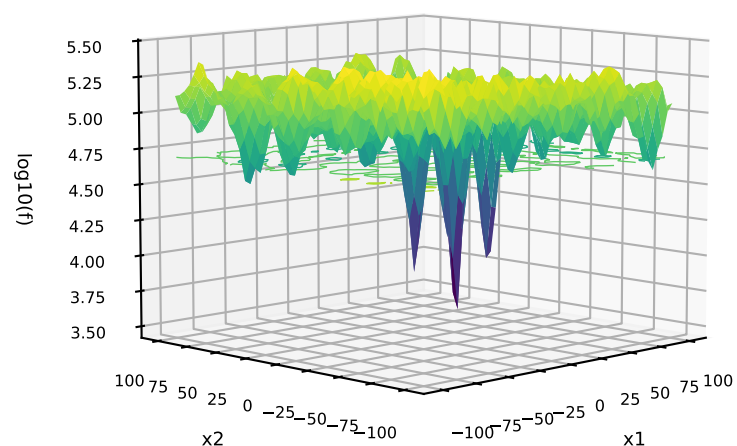
61: C=DPM-SOFTMAX; P=MIXED; T=AFF G=StyblinskiTang+Schwefel+HappyCat SchafferF7Cond1000+BuecheRastrigin
