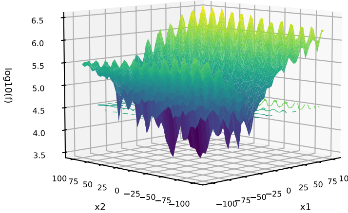
391: C=CPM-LWELL; P=MIXED; T=MIXED G=Katsuura+Gallagher21+BentCigar Gallagher21+HappyCat+Katsuura
