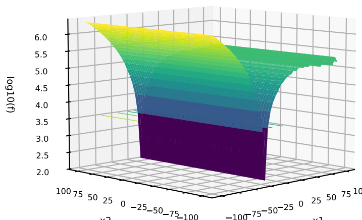
402: C=CPM-PMEAN; P=MIXED; T=MIXED G=SumDifferentPowers+LinearSlope+LinearSlope+Levy Katsuura+Weierstrass+SchafferF6+Gallagher21
