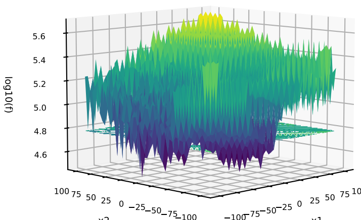
403: C=CPM-PMEAN; P=NONE; T=MIXED G=SchafferF7 Gallagher21
