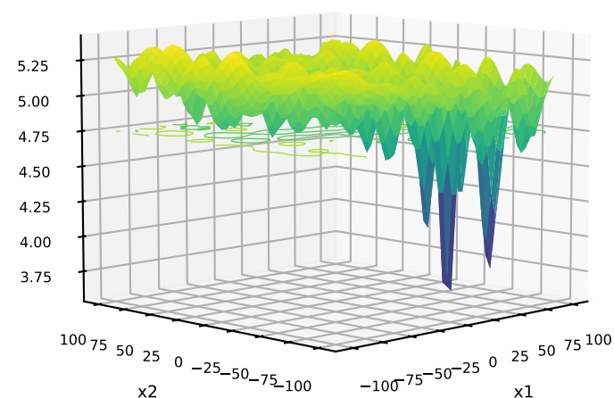
228: C=CPM-PMEAN; P=MIXED; T=AFF G=BentCigar Rosenbrock
