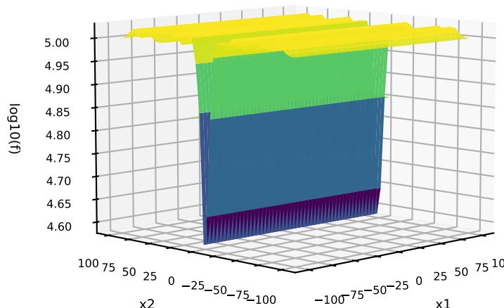
394: C=CPM-PMEAN; P=NONE; T=MIXED G=Katsuura Rastrigin
