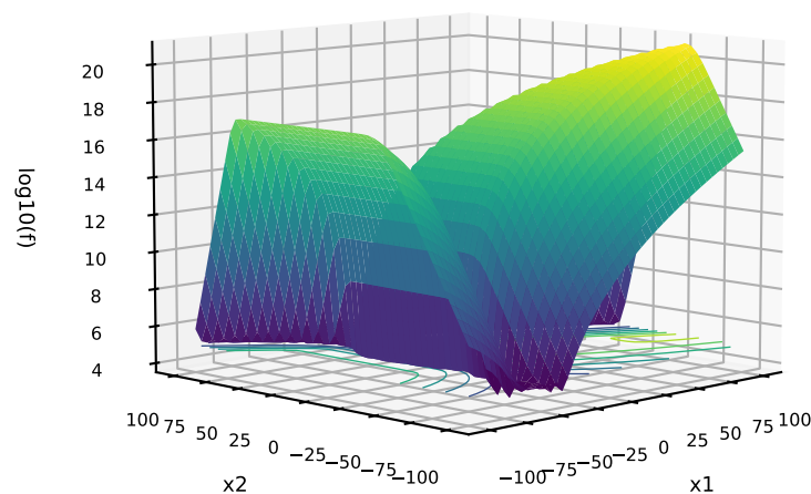
66: C=CPM-PMEAN; P=MIXED; T=MIXED G=Schwefel+SumDifferentPowers+StepRastrigin+Ellipsoidal SchafferF7Cond1000+BuecheRastrigin+SumDifferentPowers+StepRastrigin
