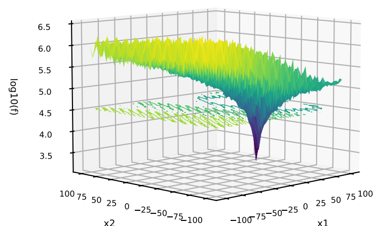
81: C=CPM-PMEAN; P=MIXED; T=MIXED G=Gallagher21 HappyCat+BentCigar
