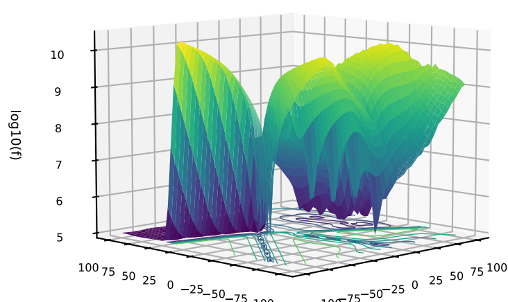
405: C=CPM-LWELL; P=MIXED; T=MIXED G=SchafferF6+Ackley+HGBat Gallagher21+Rosenbrock+HGBat
