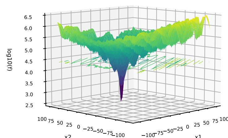
235: C=DPM-SOFTMAX; P=MIXED; T=MIXED G=SumDifferentPowers+Katsuura Exponential+SchafferF7Cond1000
