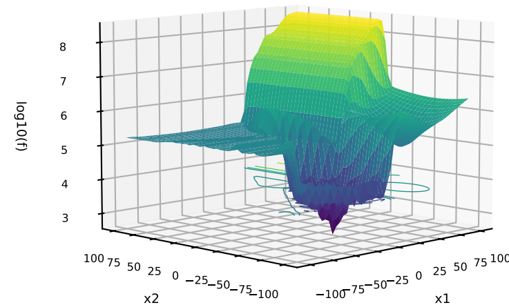
227: C=DPM-BGSOFTMAX; P=MIXED; T=MIXED G=Exponential+SchafferF6+Katsuura SumDifferentPowers+Schwefel
