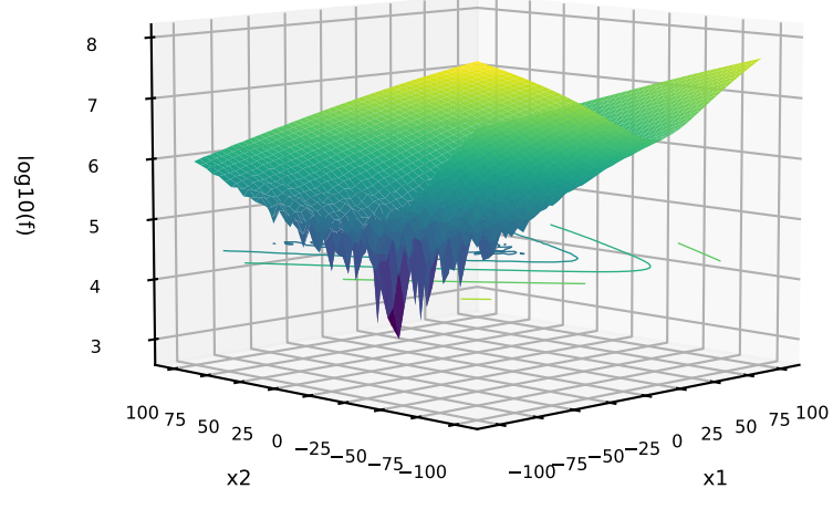
21: C=NONE; P=NONE; T=BROT G=Zakharov
