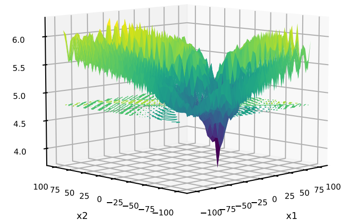
220: C=CPM-PMEAN; P=MIXED; T=MIXED G=HappyCat+Ackley SchafferF6
