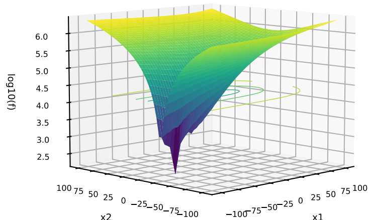
393: C=DPM-BGSOFTMAX; P=MIXED; T=MIXED G=BentCigar+BentCigar+HappyCat+GriewankRosenbrock LinearSlope+Ellipsoidal+Rastrigin
