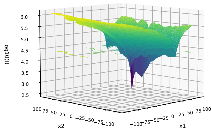
70: C=DPM-BGSOFTMAX; P=MIXED; T=MIXED G=Rastrigin Katsuura
