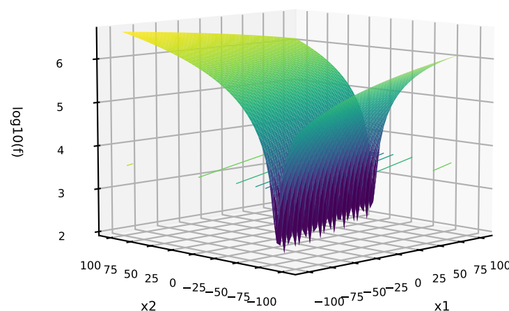
63: C=CPM-PMEAN; P=MIXED; T=MIXED G=Ellipsoidal+Exponential+SumDifferentPowers HGBat+Katsuura+Weierstrass+Gallagher21
