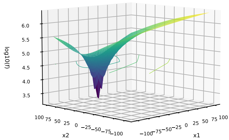
6: C=NONE; P=NONE; T=BROT G=StepEllipsoid
