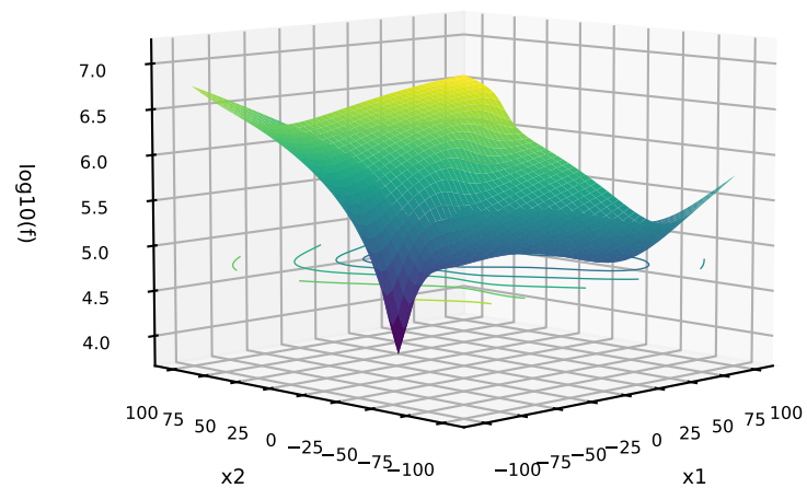
69: C=CPM-PMEAN; P=POWER; T=MIXED G=Exponential+StepRastrigin Weierstrass+Ackley
