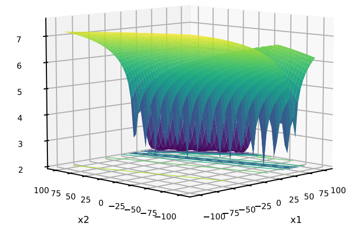
68: C=DPM-BGSOFTMAX; P=MIXED; T=MIXED G=HappyCat+LinearSlope Weierstrass+LinearSlope
