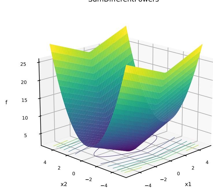
2: SumDifferentPowers
