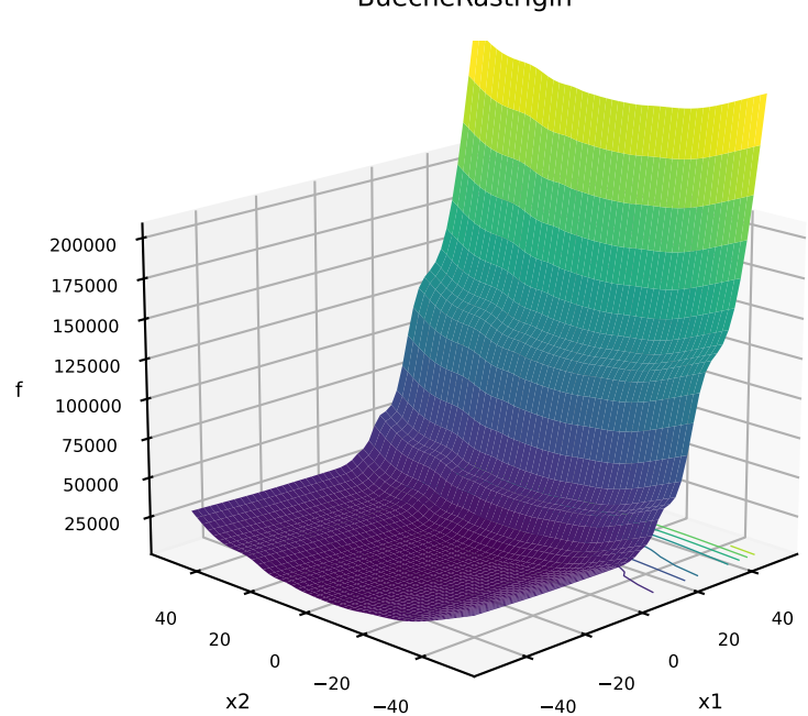
3: BuecheRastrigin
