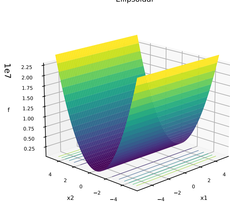
1: Ellipsoidal
