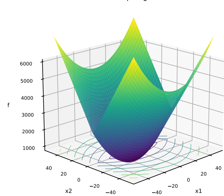
13: SharpRidge
