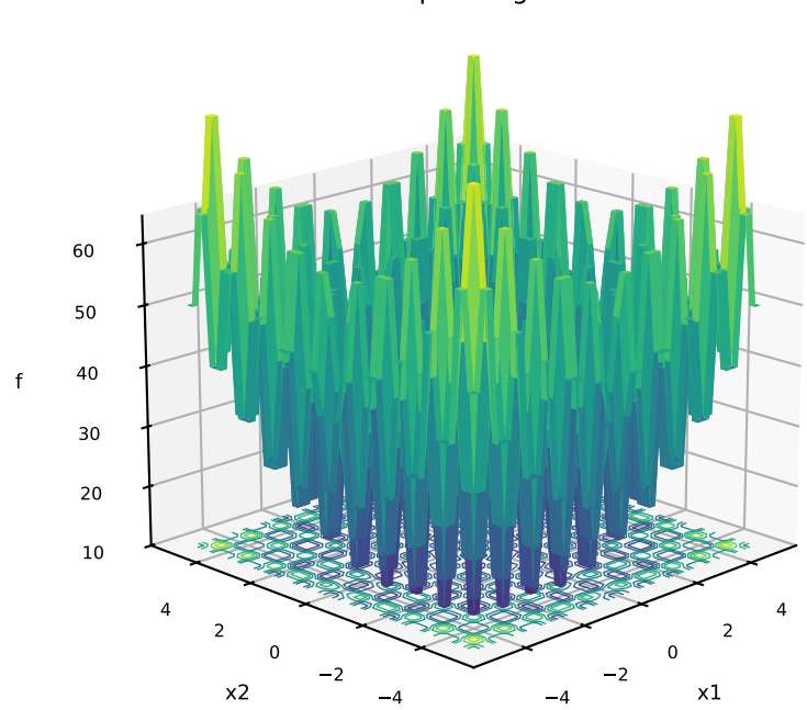
7: StepRastrigin
