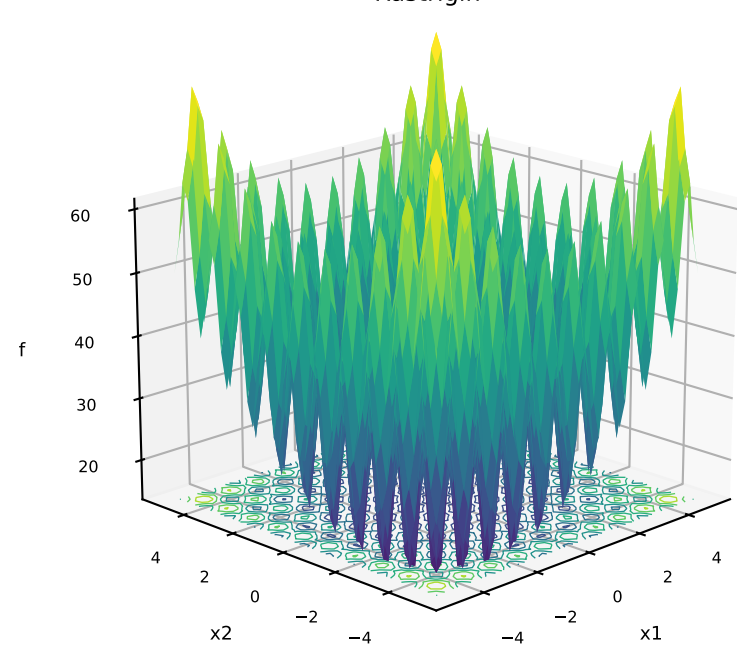
10: Rastrigin
