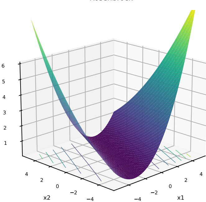
8: Rosenbrock
