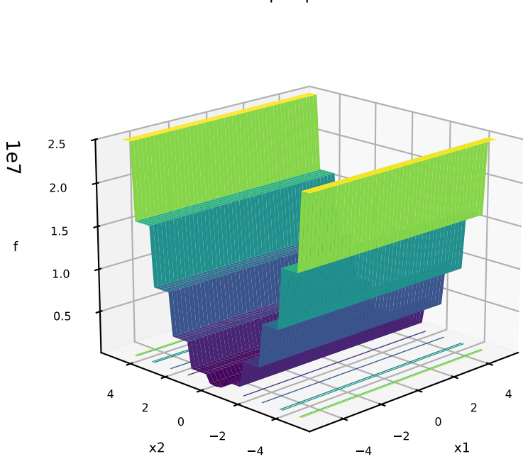
6: StepEllipsoidal
