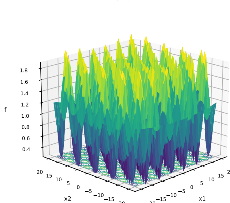
11: Griewank
