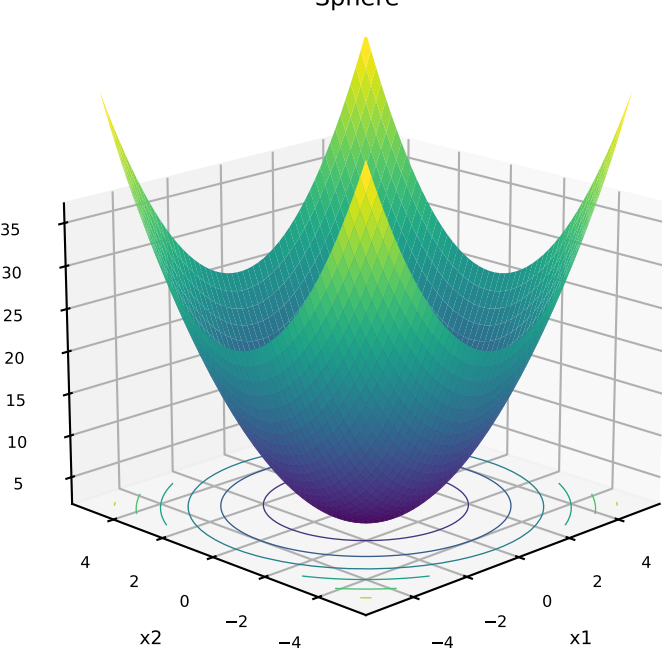
0: Sphere
