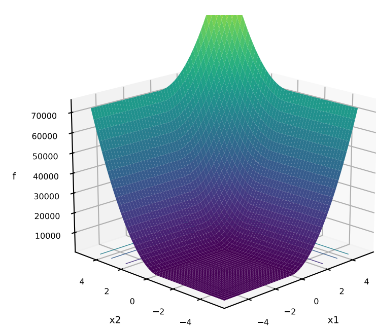
5: AttractiveSector
