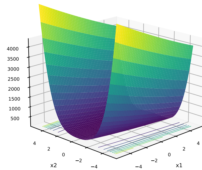
28: HCF
