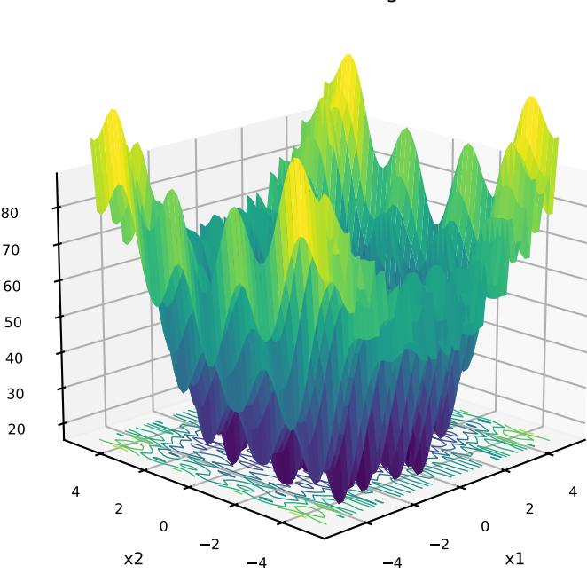
20: LunacekBiRastrigin
