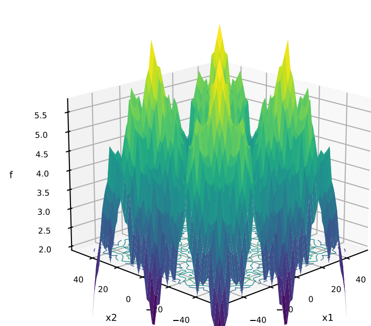
14: Weierstrass
